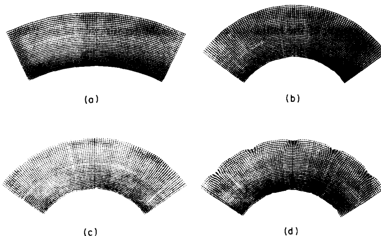
Fig. 7. The deformed mesh at four curvatures for the nonlinear elastic solid. (a) \kappa h_0 = 0.300 , (b) \kappa h_0 = 0.626 , (c) \kappa h_0 = 0.632 and (d) \kappa h_0 = 0.654 . The initial imperfection is specified by \xi_1 = 0.0006 , m = 1 and \xi_2 = 0 in (8), with a half wavelength to initial thickness ratio of 0.301. The configuration shown is for a plate five wavelengths long, but only one half wavelength was analyzed numerically.
