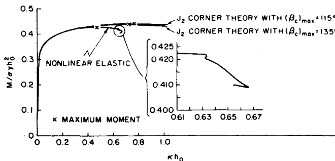
Fig. 4. The moment, M , vs curvature, \kappa h_0 , relations for plates with the initial thickness inhomogeneity specified by \xi_1 = 0.0006 , m_1 = 1 and \xi_2 = 0 in (8), with a half wavelength to initial thickness ratio of 0.301.
